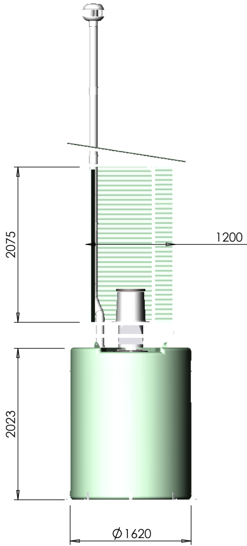
FRONT VIEW
