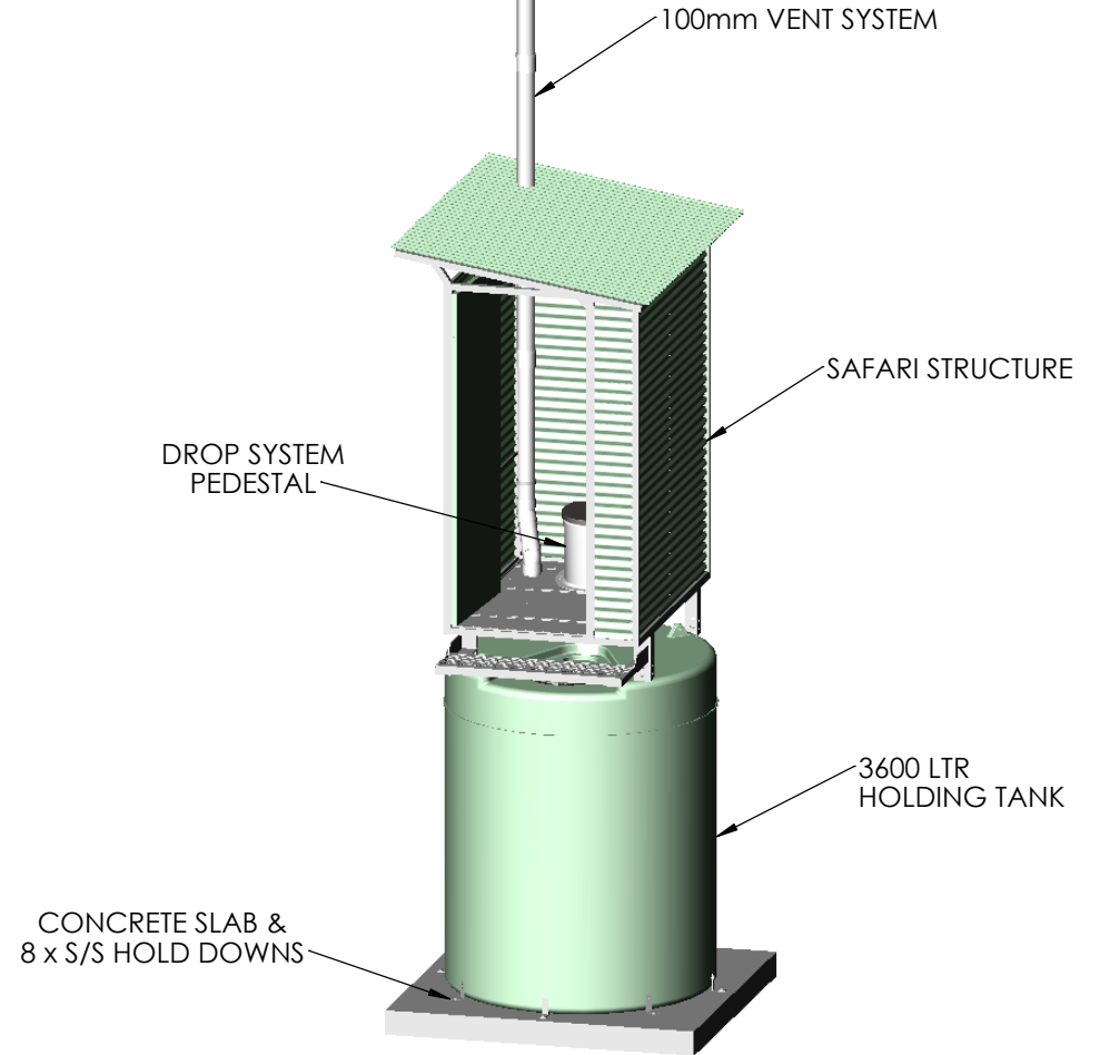
DIMETRIC VIEW
