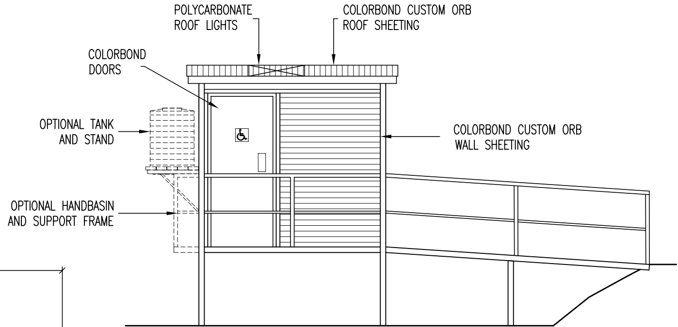
FRONT VIEW (1:50)
